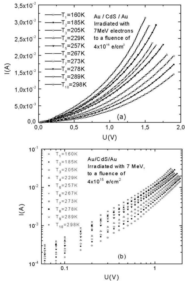
Fig. 4. The I-U characteristics for the Au/CdS/Au cells irradiated with 7 MeV electrons to a fluence of 4 \times 10^{15} \text{ e/cm}^2 , for different temperatures: (A) in linear scale; (B) in logarithmic scale.
