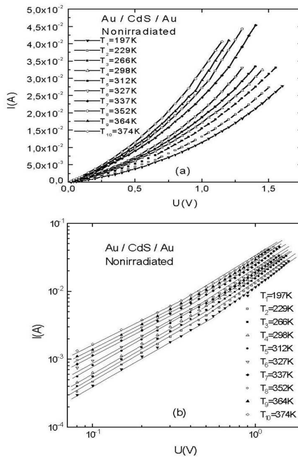
Fig. 2. The I-U characteristics of nonirradiated Au/CdS/Au cells for different temperatures: a) in linear scale; b) in logarithmic scale.
