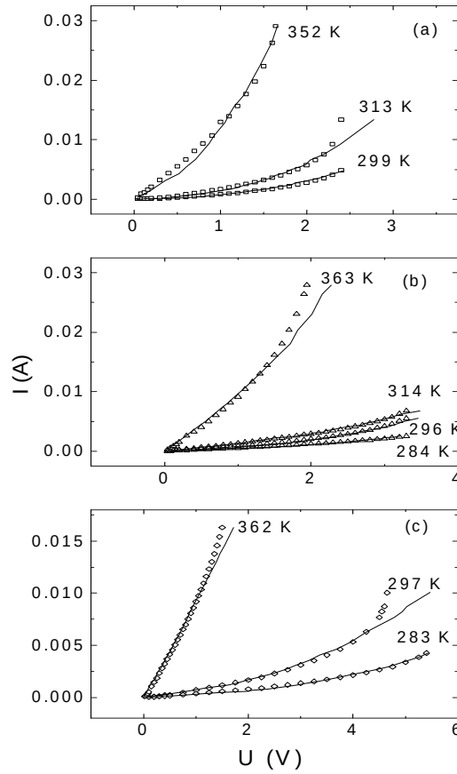
Fig. 10. Current-voltage characteristics at different temperatures, before (a) and after the first (b) and second (c) irradiation sessions. Both the measured values (points) and the best fits (continuous line) obtained as indicated in text are plotted.
