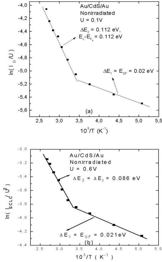
Fig. 3. a) Dependence of \ln(I_Q / U) on the reciprocal temperature 10^3/T at U = 0.1 V; b) Dependence of \ln(I_{SCLC} / U^2) on reciprocal temperature 10^3/T at U = 0.6 V, for the Au/CdS/Au structures.
